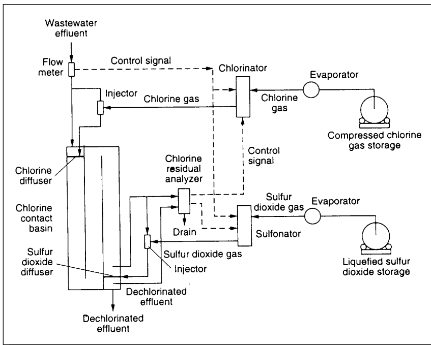
Figure 1: A compound-loop control system for chlorination with liquid chlorine and dechlorination with sulfur dioxide
