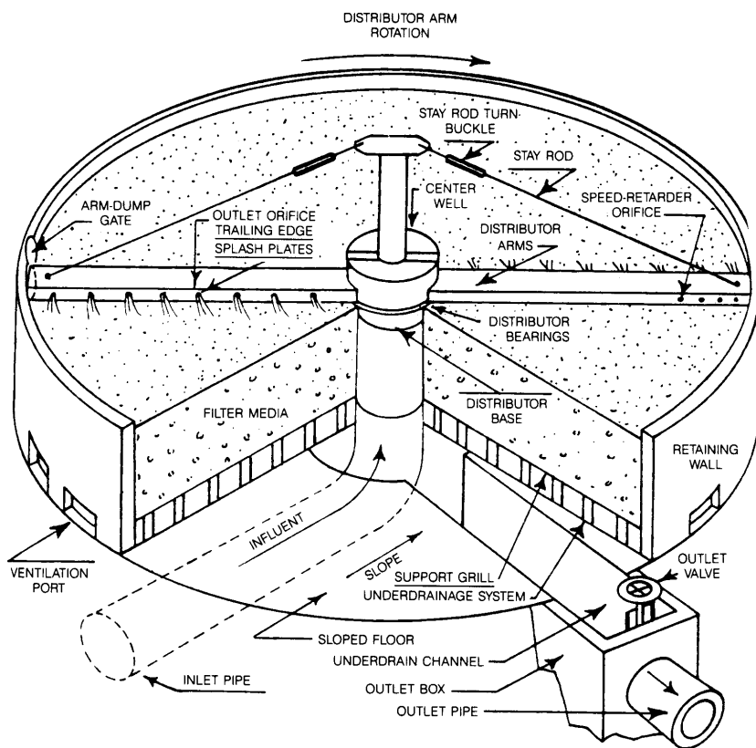
Figure 1: Schematic of a Trickling Filter
